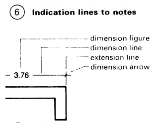
7 Designation for dimensioning
